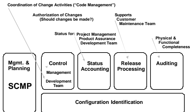
Figure 1. SCM Activities
