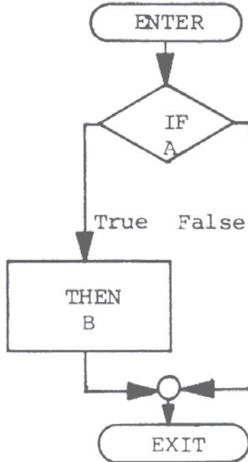
Figure 2 IF-THEN-ELSE
