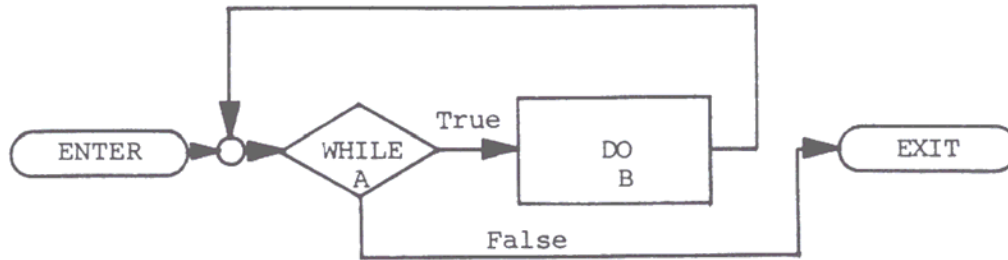
Figure 3 DO-WHILE
